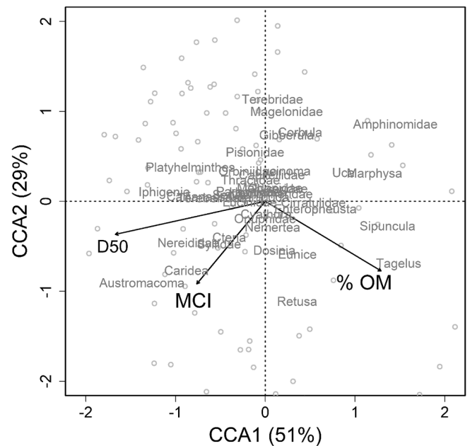
Fig. 4. Constrained correspondence analysis (CCA) of the abundance of 95% most common benthic species found in a largescale survey at Bijagós Archipelago and the environmental variables that have statistically ( P < 0.05 ) affected the community assemblages. MCI = mangrove connectivity index, D50 = sediment median grain size, % OM = sediment organic matter content.
