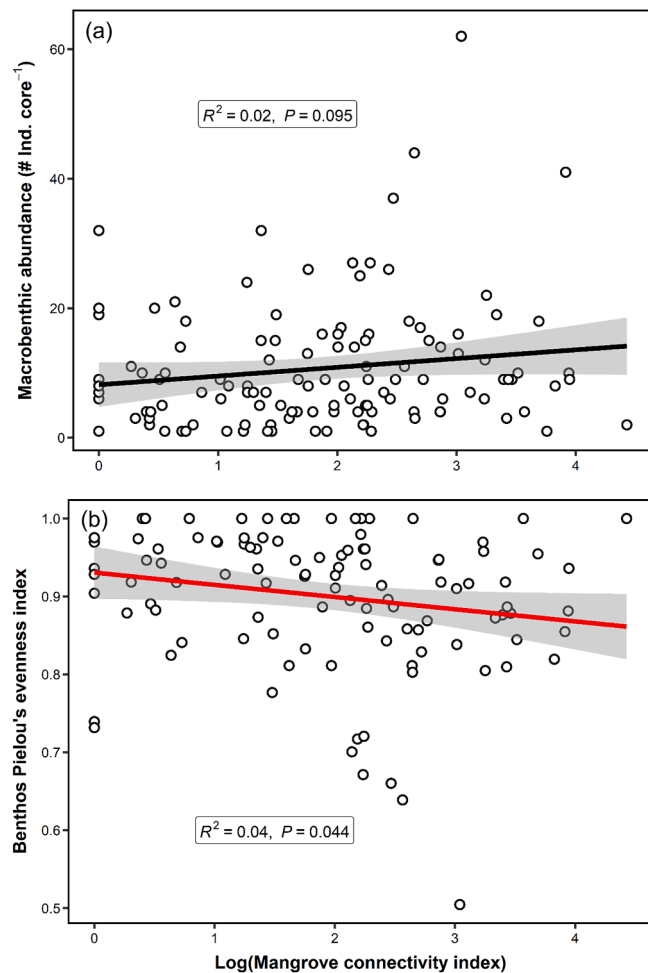
Fig. 3. Relationships between mangrove connectivity index and benthic community structure: (a) benthic total abundance, (b) benthic community evenness. The black line denotes a positive trend while the red line depicts a negative trend. 95% Confidence intervals are depicted in grey. (For interpretation of the references to colour in this figure legend, the reader is referred to the web version of this article.)
