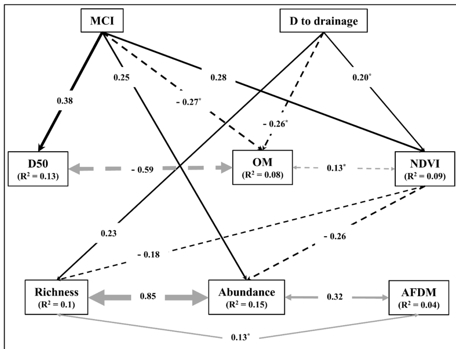
Fig. 5. The final piecewise structural equation model (Fisher's C statistic = 15.65, P = 0.99 ), depicting the effects of environmental variables (Mangrove connectivity index (MCI), distance to drainage, sediment median grain size (D50), and NDVI) on macrobenthic richness, abundance, and total biomass (AFDM). The width of arrows is proportional to the path coefficient, with solid lines represent positive causal links, dashed lines negative links, and grey arrows non-causal correlations. The R^2 value indicates the amount of variance explained by the model. The final model included only significant and almost significant pathways ( 0.05 > p < 0.1 ; indicated by * pathways). Distance to subtidal was removed as this was not included in any significant pathway.
