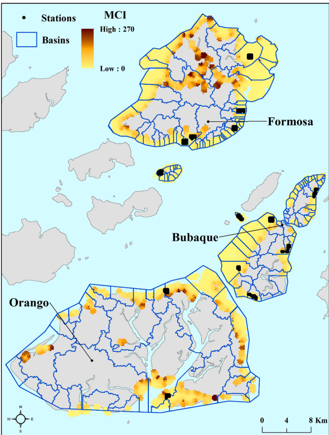
Fig. 2. Interpolated mangrove connectivity index (MCI) map of the mudflats using inverse distance weighing tool in ArcGIS (Spatial Analyst Tools) with sampling stations (black dots) and studied basins (blue outlines) delineated using a digital elevation model (DEM) image (~10 m resolution; SRTM v3, U.S. Geological Survey) and modelled in ArcGIS (Spatial Analyst Tools). (For interpretation of the references to colour in this figure legend, the reader is referred to the web version of this article.)
